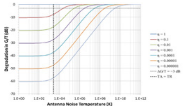
Fig. 1. G/T degradation versus antenna noise temperature for T_R = 2610 K (i.e. 10 dB noise figure) and T_{AP} = 290 K.
