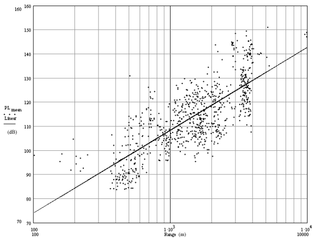
Figure 1. Example BS mean path-loss measurements and linear fit
