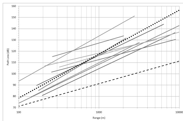
Figure 5. Comparison of Hata model (dotted line) with least-squares approximation of mean path loss for all BS analysed (free-space path loss shown as dashed line)
