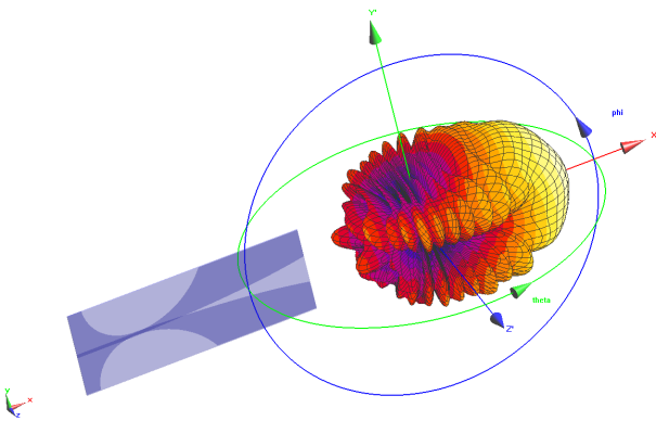
Figure 3. Simulated 3D radiation pattern at 22 GHz
