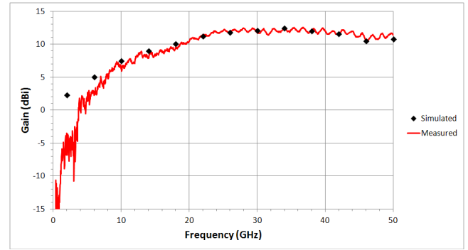
Figure 5. Simulated and measured forward gain
